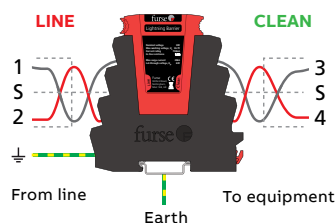
ESP SL30L/4-20 installation
