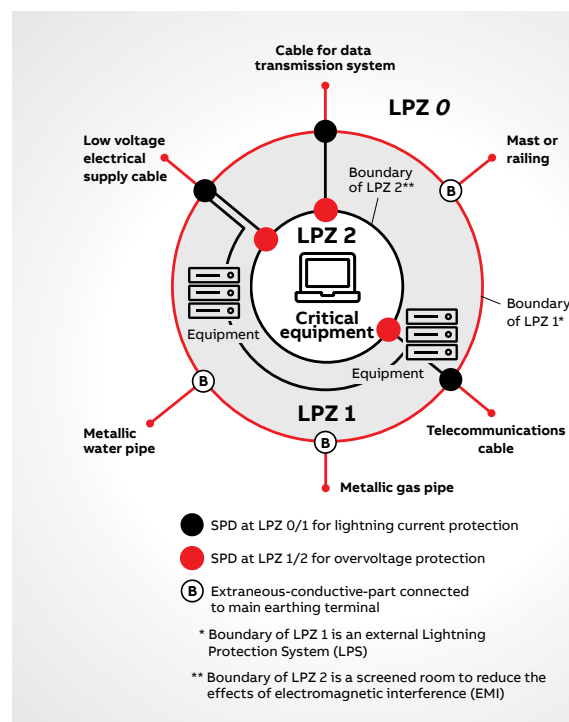
Figure 1 – Basic LPZ concept - IEC/ BS EN 62305-4
