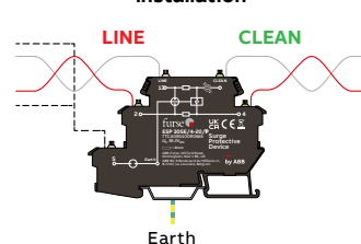
ESP SE30/4-20/PT installation
