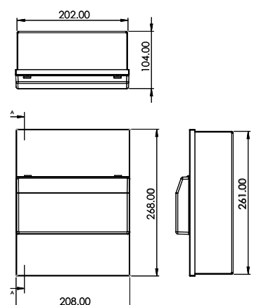
Dimensions (mm) MBX D8
